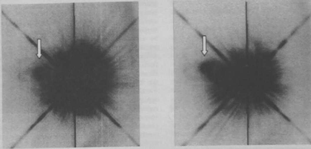
HST Archive images of the DG Tau jet taken in September 1995 and February 1998 (left and right image respectively) showing the expansion in the Herbig-Haro flow. The position of the Herbig-Haro bowshock is indicated by means of an arrow in both frames.
