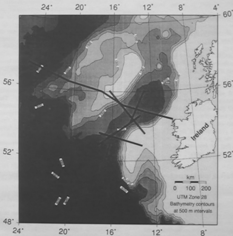
RAPIDS offshore seismic lines
