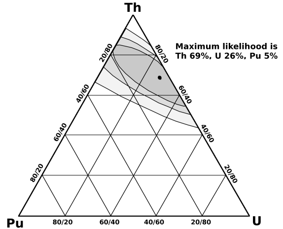
Figure 1: Likelihood contours (at the 90%, 70% and 50% levels) for a ternary U/Th/Pu composition of the actinides in the GCR as derived from the UHCRE data.
