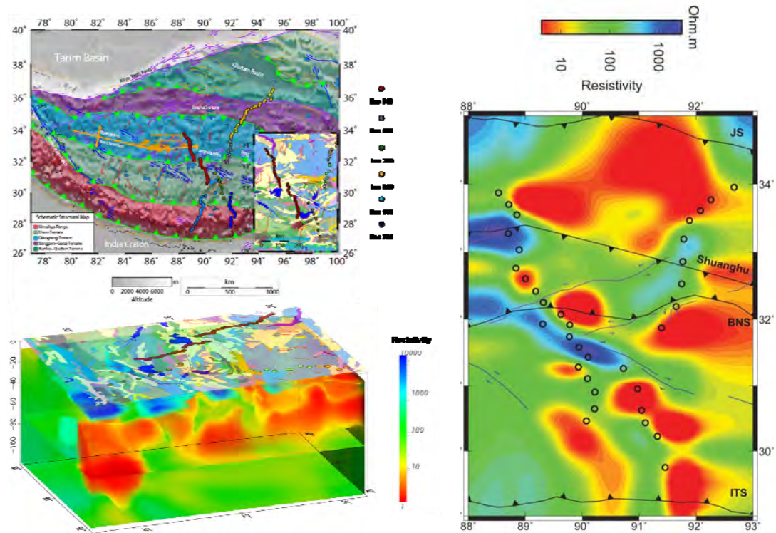
Figure 1: MT 3D final model visualisation with horizontal slice at 50km with surface strike-slips faults and sutures
