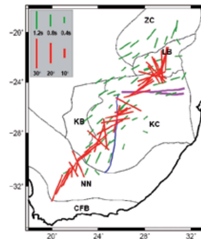
Figure 3.1.5: Electrical more conductive directions (in red), scaled by maximum phase difference, for the lithospheric upper mantle, and the shear-wave-splitting results (both high and low quality results plotted in green, but sites with no detectable splitting omitted) from Hamilton et al. (2006). ZC: Zimbabwe craton. KC: Kaapvaal craton. LB: Limpopo Belt. NN: Namaqua-Natal mobile belt. CFB: Cape Fold Belt. KB: Kheis and Proterozoic fold and thrust Belt. Blue line: the N-S trending Colesburg Magnetic Lineament (CML). Purple lines: the E-W trending Thabazimbi-Murchison Lineament (TML).
