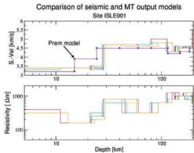
Figure 2.4.1: Joint inversion models of data from a site in southern Ireland. The model marked "Prem" is the global standard 1D velocity model of the Earth.
