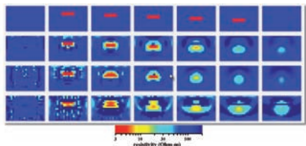
Figure 3.4.1: Results of the inversions. Each row of panels presents seven horizontal (x-y) slices of the model starting from 150 m (left) to 750 m (right) depth (z). 1st row corresponds to the true model; 2nd row – to the result of the inversion with use of the stabilizer and with gradually diminishing regularization parameter; 3rd row – to the result of the inversion when we restart the inversion every 20 iterations and without use of the stabilizer, and the last row corresponds to the result of the inversion without use of the stabilizer, but with limits imposed on conductivities.
