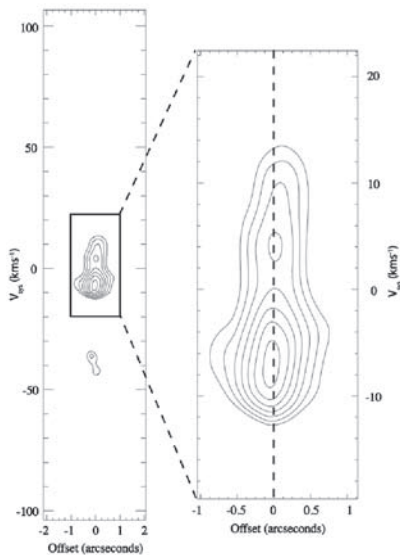
A position velocity diagram of the 2MASS1207-3932 bipolar outflow in the [O I] \lambda 6300 line. The blue and red-shifted lobes are detected at radial velocities of -8/+4 \text{ km s}^{-1} respectively (with respect to the systemic velocity).
