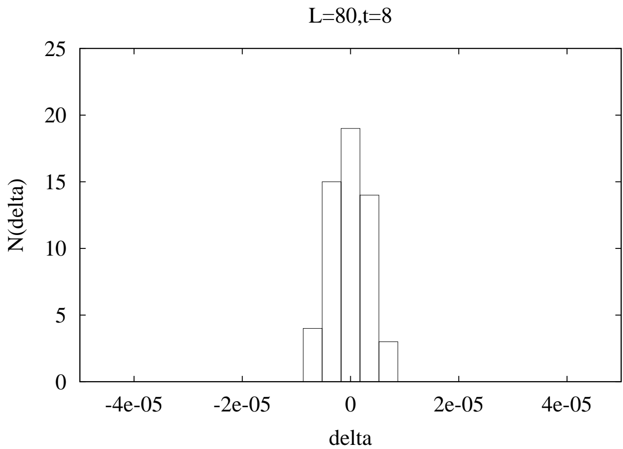
Figure 3: Histogram of \Delta(R_1, R_2) for all the values of R_1, R_2 \geq 20 . Notice the very small scale of the \Delta axis.
