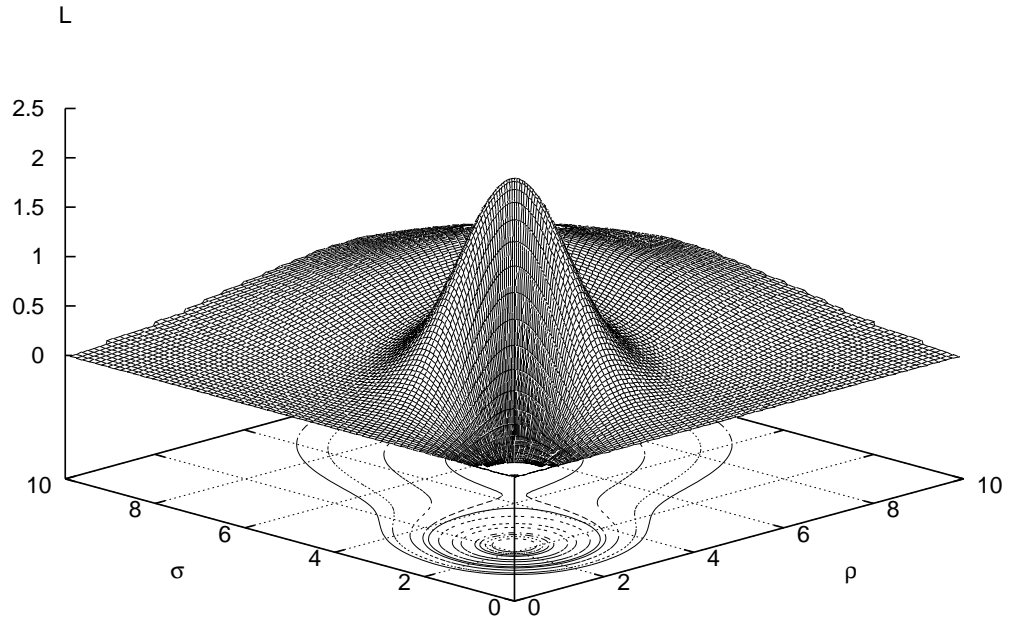
m=2, n=2 lower 2-nodes branch: Action density at \alpha=0.2
