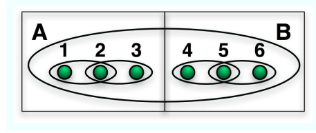
FIG. 1: A Bell type measurement on six particles. First a joint measurement (large oval) on all six particles is made and the result kept if the total charge (or spin) is zero. Alice performs measurements of total charge on pairs 1,2 and 2,3 and Bob performs measurements on pairs 4,5 and 5,6. For some quantum states the correlator \langle W \rangle exceeds the bound set by local hidden variable theories.
