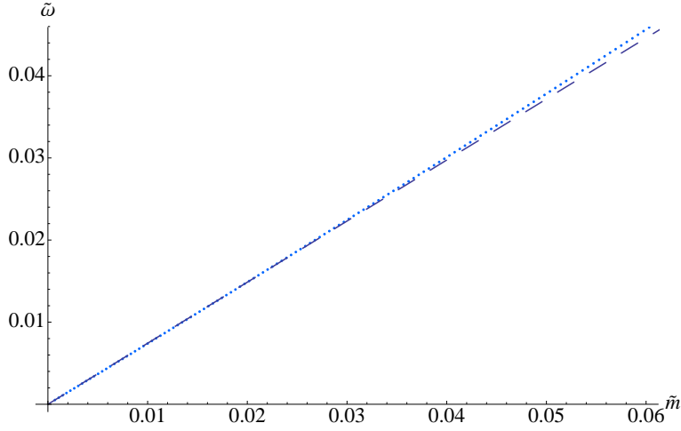
Figure 10: Plot of the spectrum of the ground state from figure 9 for small bare masses. The dashed line corresponds to the linear behavior from equation (4.189).
