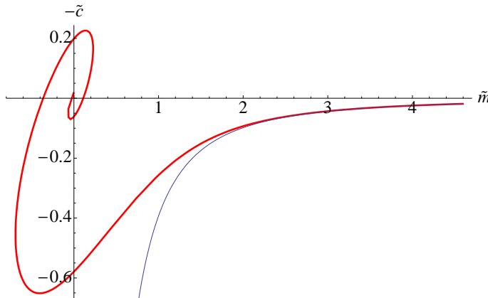
Figure 7: A plot of -\tilde{c} vs. \tilde{m} . At zero bare mass \tilde{m} = 0 the theory has developed a negative condensate \langle \bar{\psi}\psi \rangle \propto -\tilde{c}_{\text{cr}} \approx -0.59 . For large \tilde{m} there is excellent agreement with equation (4.167), as represented by the lower (blue) curve.
