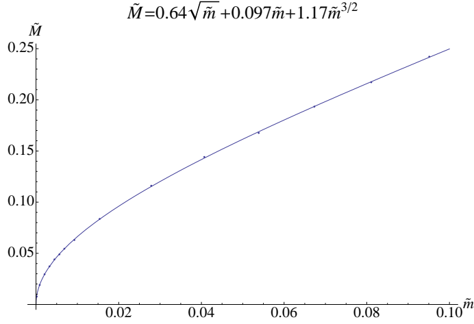
Figure 6: There is a characteristic \tilde{M} \propto \sqrt{\tilde{m}} behavior at small bare quark mass.
