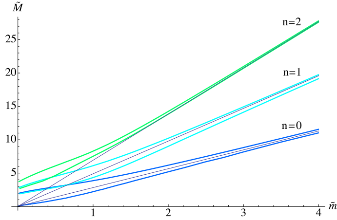
Figure 5: There is Zeeman splitting of the states due to the magnetic field. In the absence of the field there are three straight lines emanating from the origin; these are split to form six curves. At zero bare quark mass (the end of the lowest curve) there is indeed a massless Goldstone mode. The straight lines correspond to the asymptotic AdS results.
