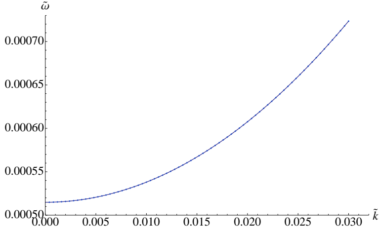
Figure 11: Plot of the dispersion relation of the pseudo-Goldstone mode for \tilde{m} \approx 0.0007 . The parabolic fit corresponds to equation (4.192).
