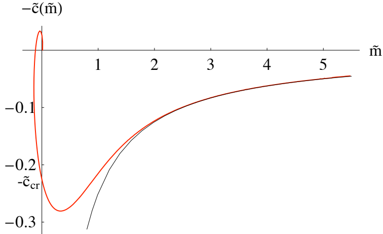
Figure 2: Parametric plot of \tilde{c} against \tilde{m} for fundamental matter in the presence of an external magnetic field. The lower (black) line represents the curve 1/\tilde{m} , fitting the large \tilde{m} behavior. It is also evident that for the outer branch of the spiral, for \tilde{m} = 0 the condensate, \langle\bar{\psi}\psi\rangle is non-zero. The corresponding value of the condensate is \tilde{c}_{\text{cr}} = 0.226 .
