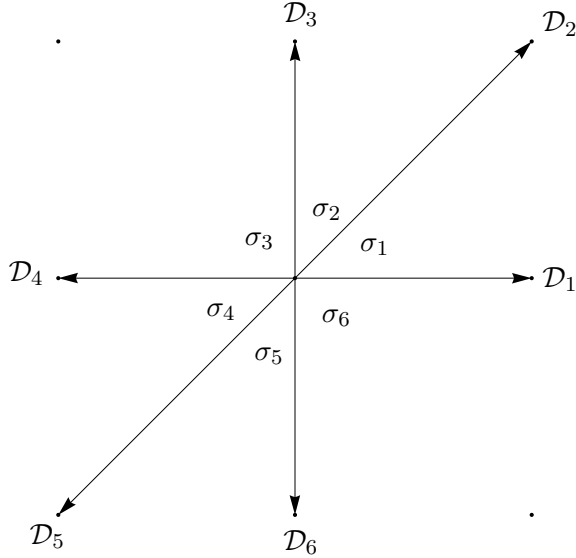
Figure 1: The fan for d\mathbb{P}_6 , with the rays labelled by the corresponding toric divisors. The two-dimensional cones \sigma_a are also labelled.
